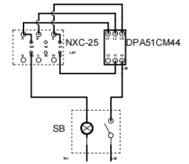
System startup contactor wiring diagram
