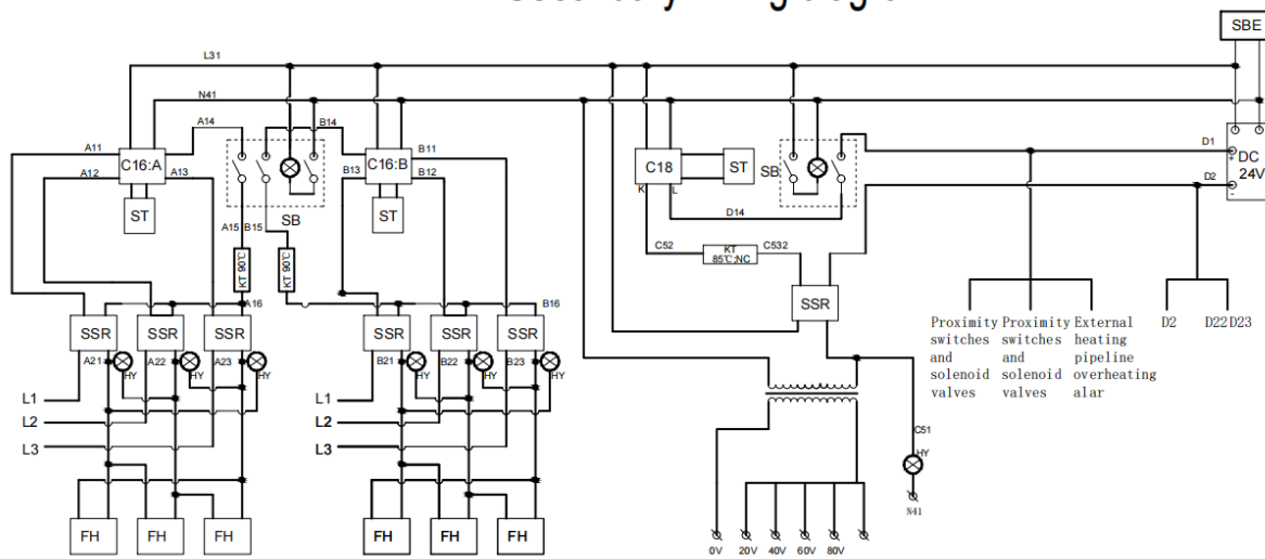
Secondary wiring diagram
