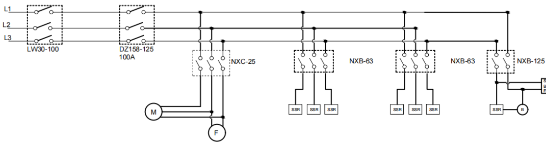
System startup contactor wiring diagram
